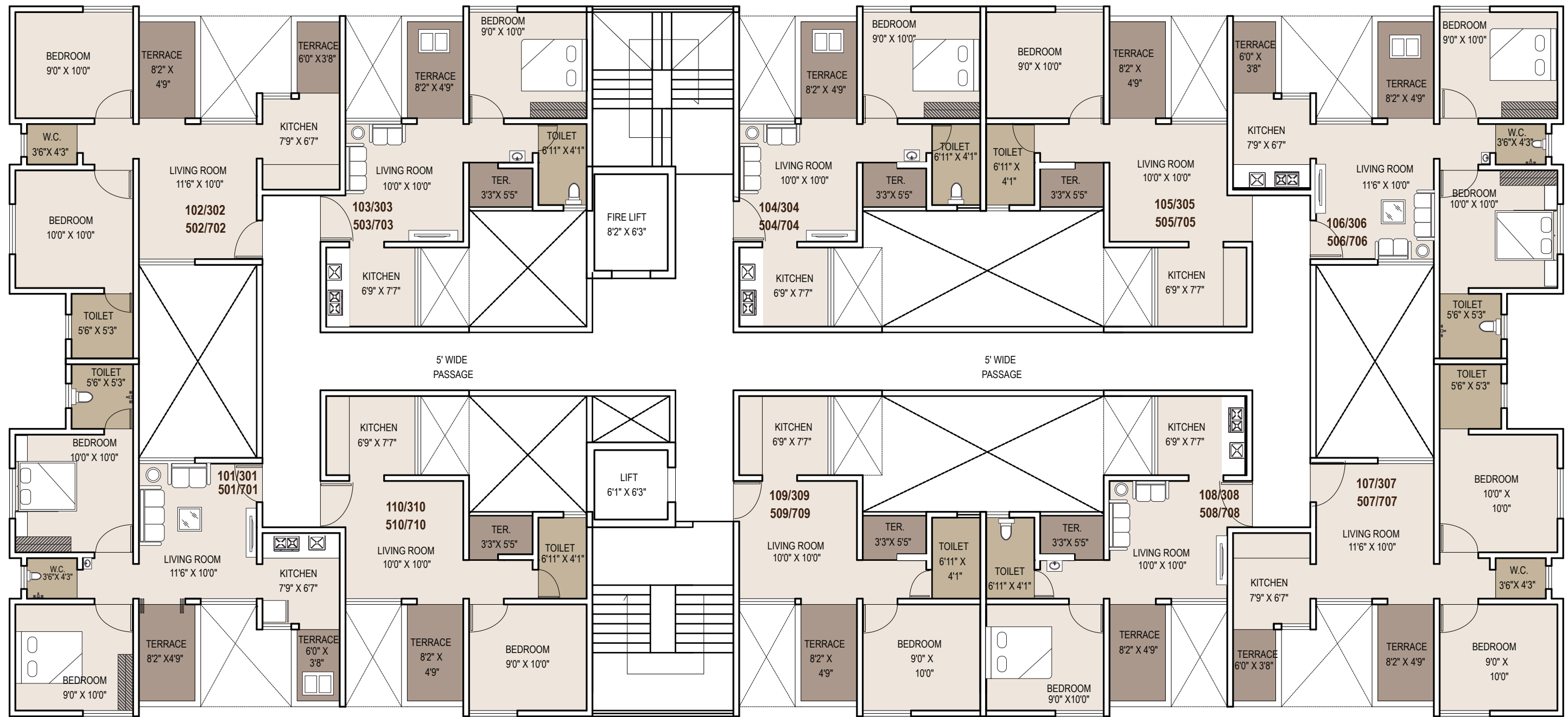
(A BLDG) - 1ST, 3RD, 5TH, 7TH FLOOR PLAN
