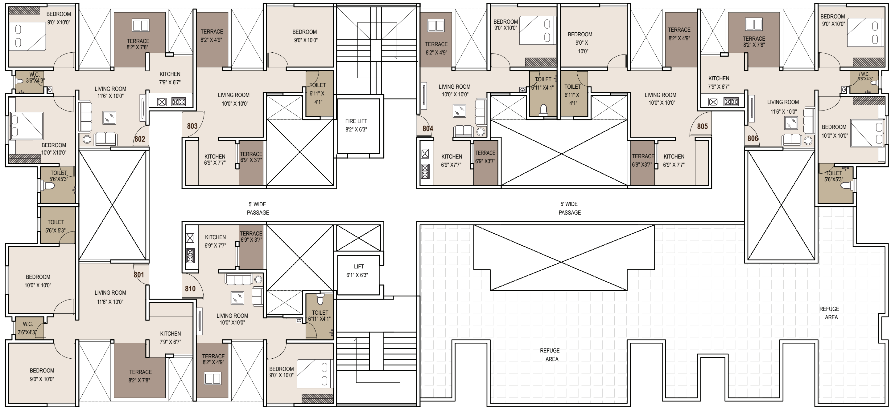
(A BLDG) - 8TH FLOOR PLAN
